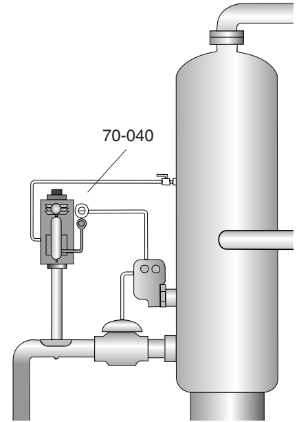
Typical configuration in use of the 70-040 Heater Regulator Drip Package
